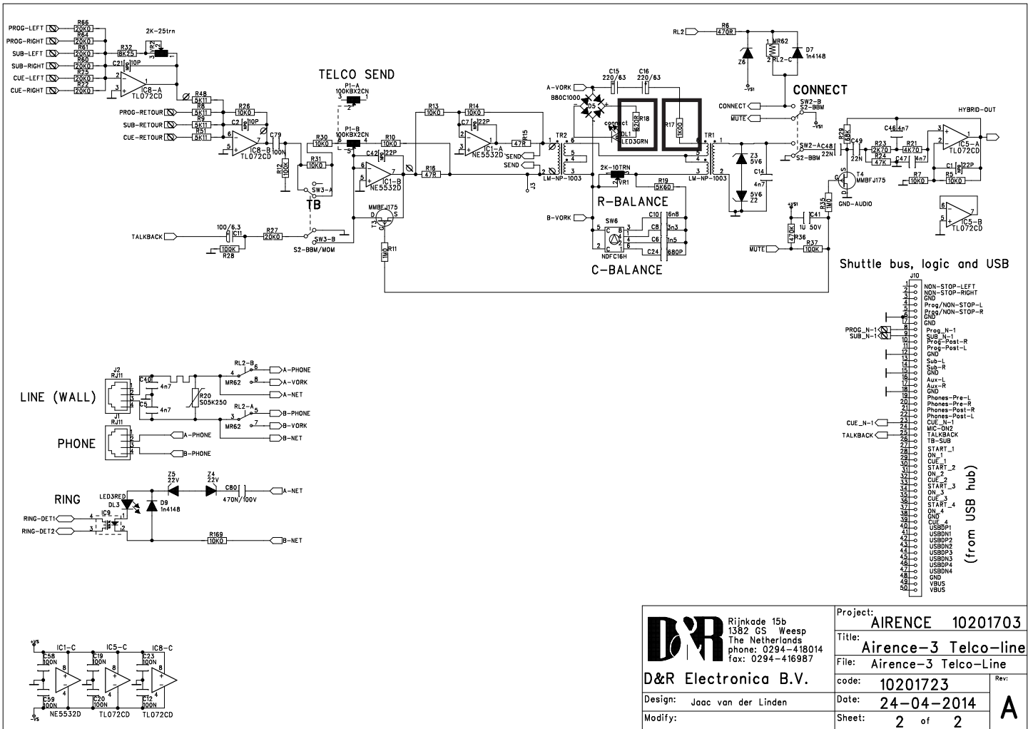
Schematic of the Hybrid with R17 and R18 to identify its place in the circuit.
